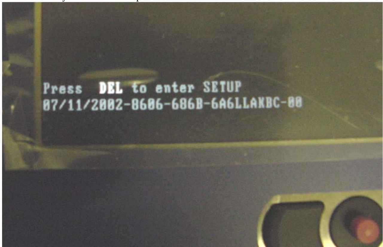
Figure 41: Entering BIOS
