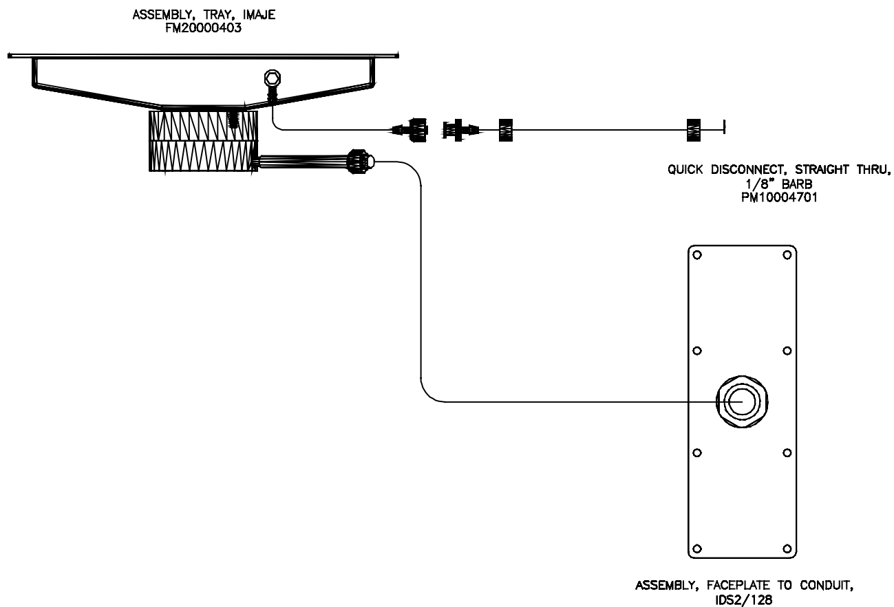
Figure 137: Plumbing Diagram, IDS2/128 (PM30000501)
