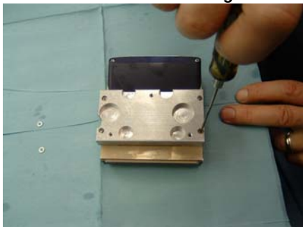
Figure 86: Place Printhead Upside Down
