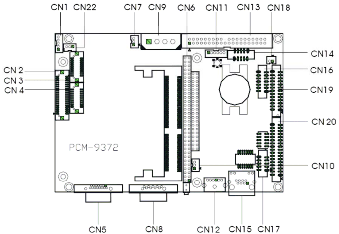
Figure 31: CPU PCB Component Side
