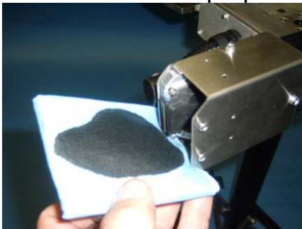
Figure 112: Blot Excess Ink Off Printhead
