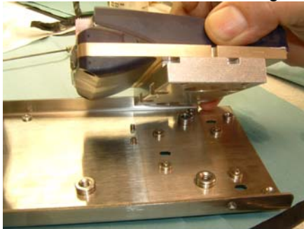
Figure 85: Assure Forward Positioning When Reinstalling
