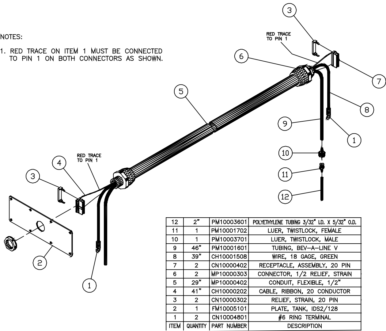
Figure 136: Exploded Drawing: Umbilical Assembly, IDS2/128 (CH20000801)
