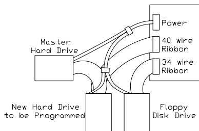
Figure 62: Master Drive at the End of Flat Cable
