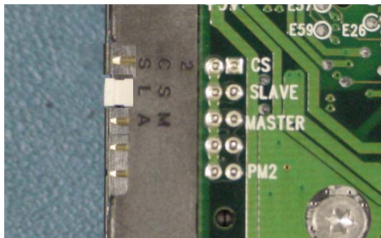
Figure 59: Set Drive as Slave
