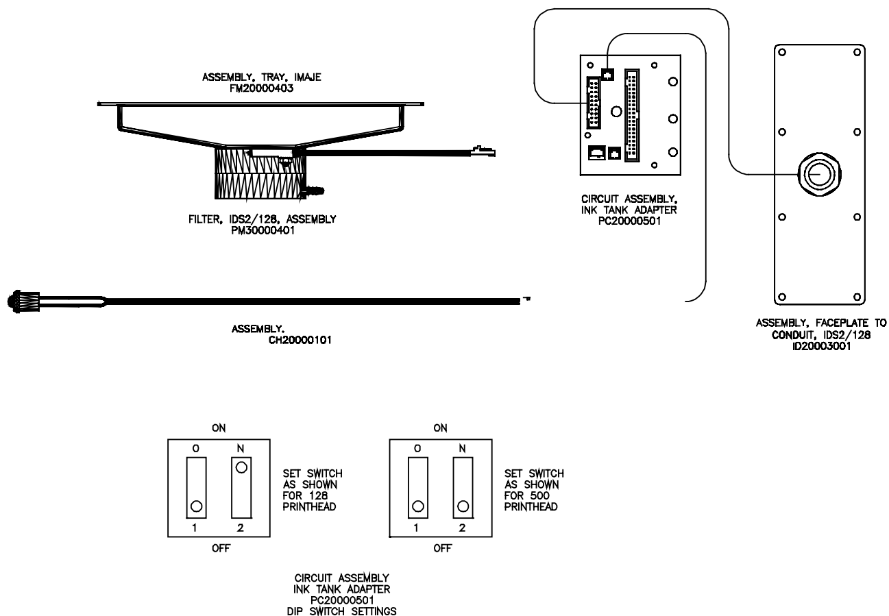
Figure 138: Electrical Diagram, IDS2/128 (ES20000201)
