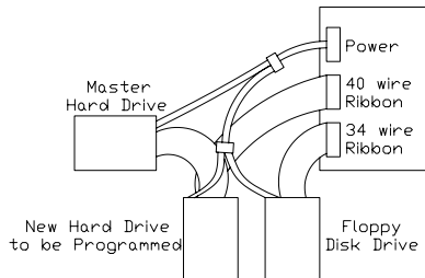
Figure 61: Connect Hard Drive
