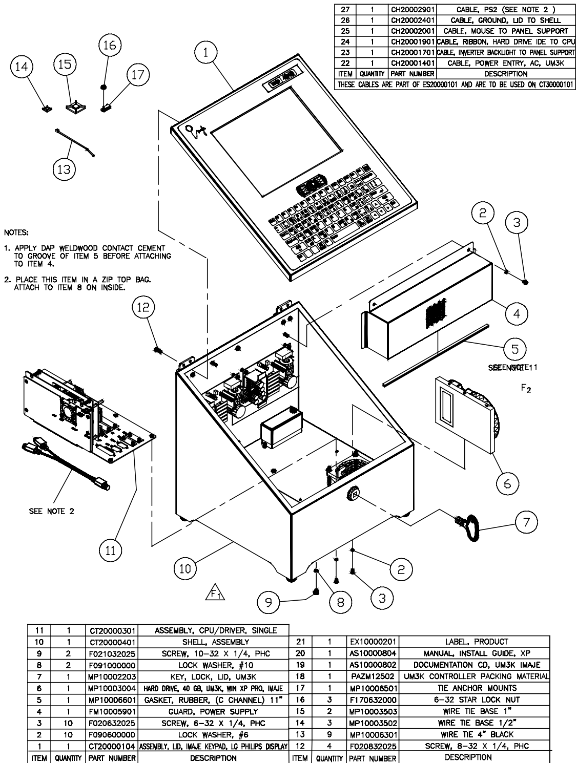
Figure 13: Exploded Drawing: Controller, Major Sub-Assembly (CT30000101)
