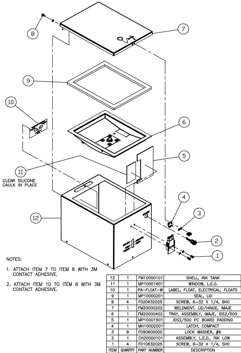
Figure 99: Exploded Drawing: Tank Shell Assembly, IDS2/500 (ID20000202)
