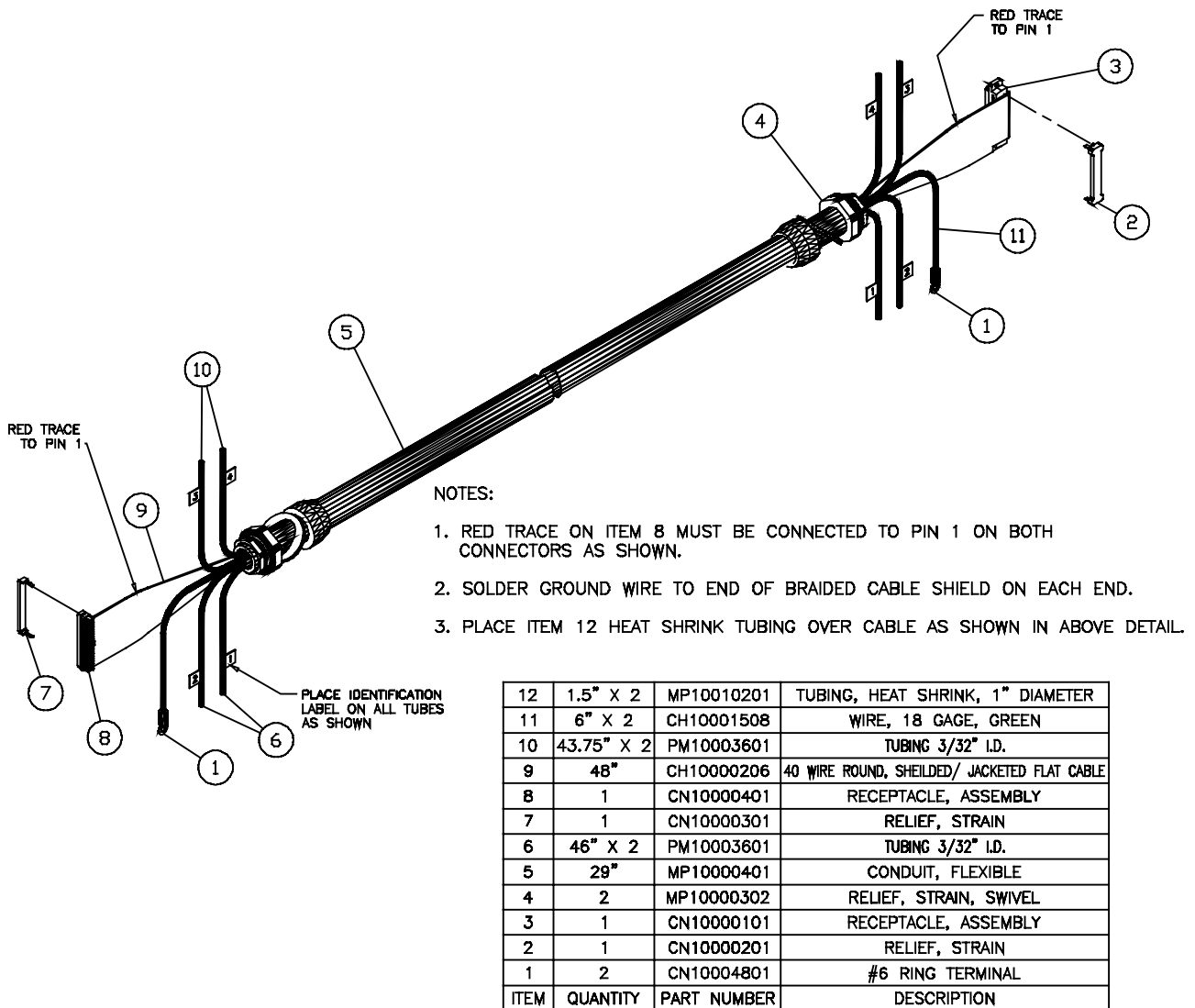
Figure 94: Drawing, Printhead Umbilical, XJ500 (CH20000201)
