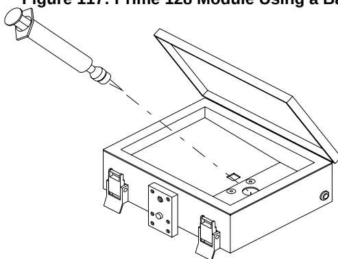
Figure 118: Prime 128 Module Using a Syringe
