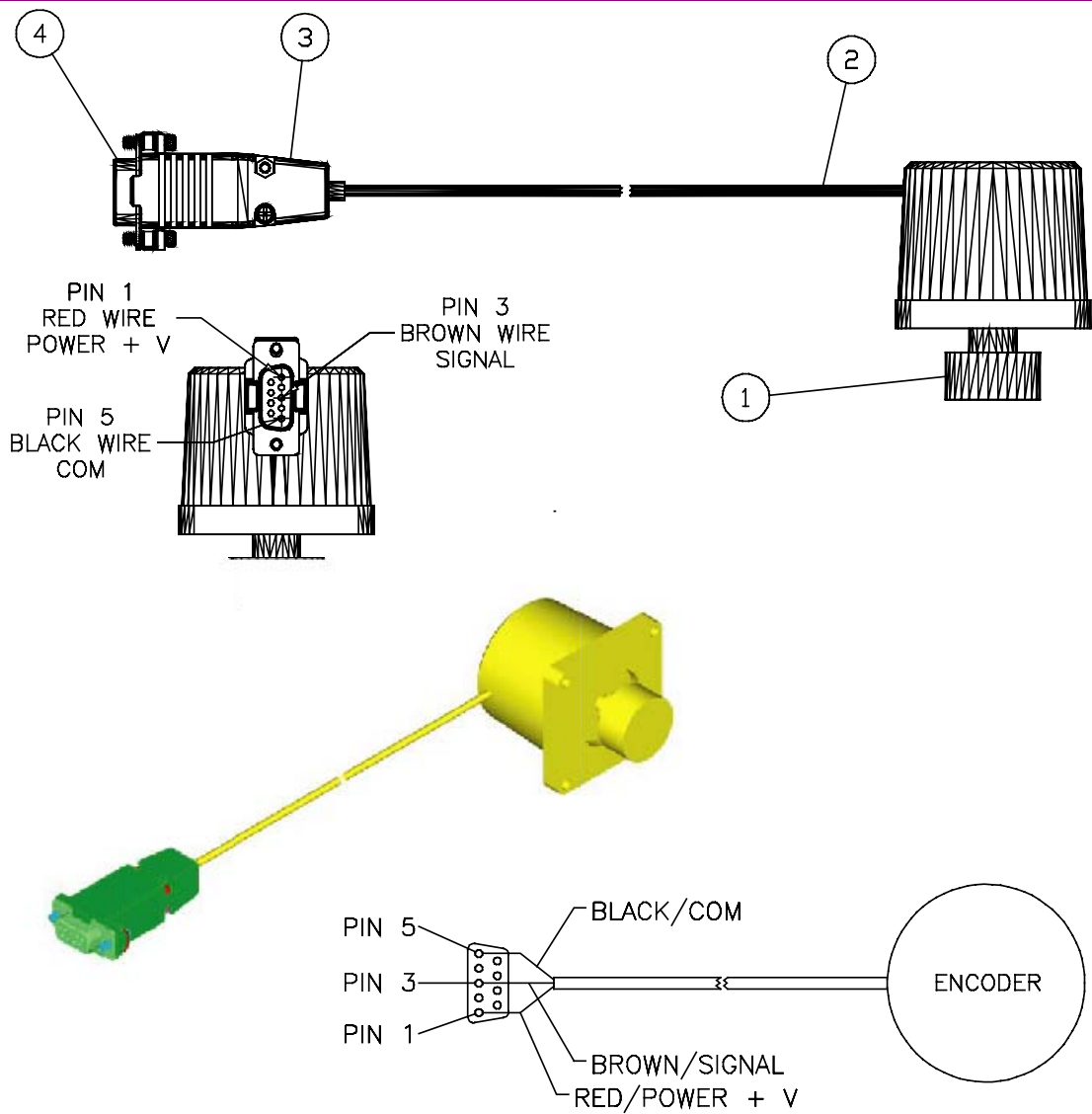
ELECTRICAL SCHEMATIC OF ASSEMBLY
