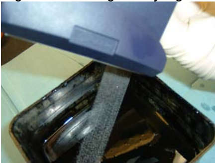
Figure 90: Cleaning Solution Streaming from Head
