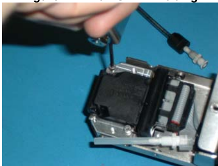
Figure 122: Remove Screws Holding 128 Printhead
