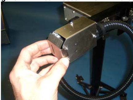
Figure 113: Re-attach Nozzle Plate
