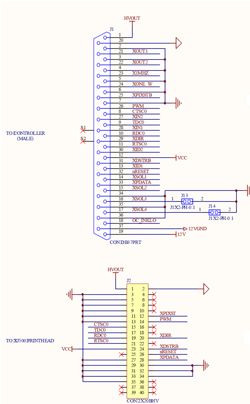
Figure 91: IDS2-500 Ink System Circuit Board Schematic, I/O
